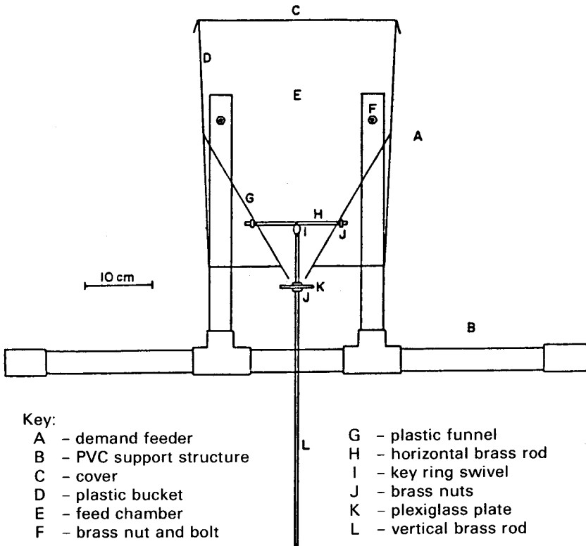
Figure 1. Cross-sectional view of demand feeder with side view of support structure superimposed.
