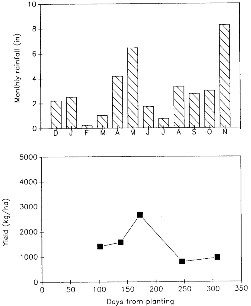
Figure 1. Yield of alfalfa in relation to rainfall.
