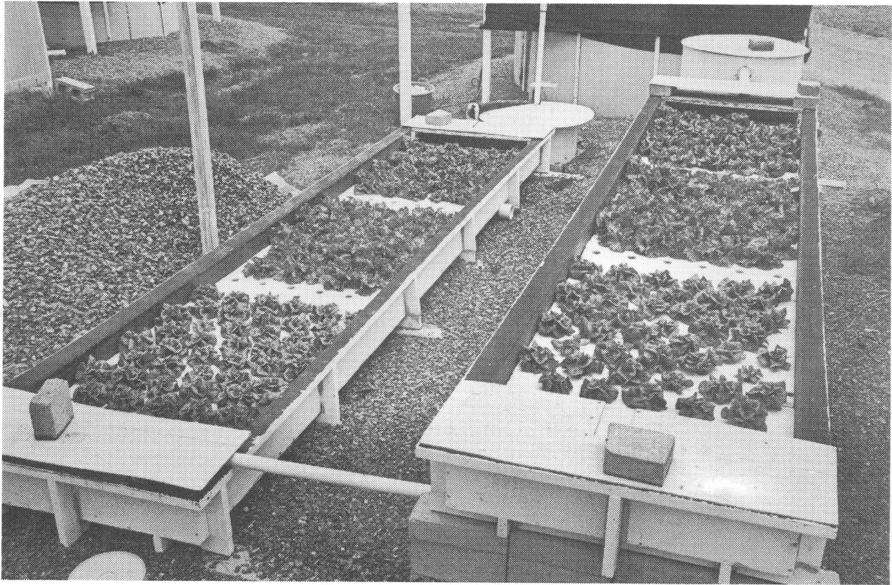
Figure 1. Hydroponically grown lettuce in a recirculating system integrated with fish culture.
