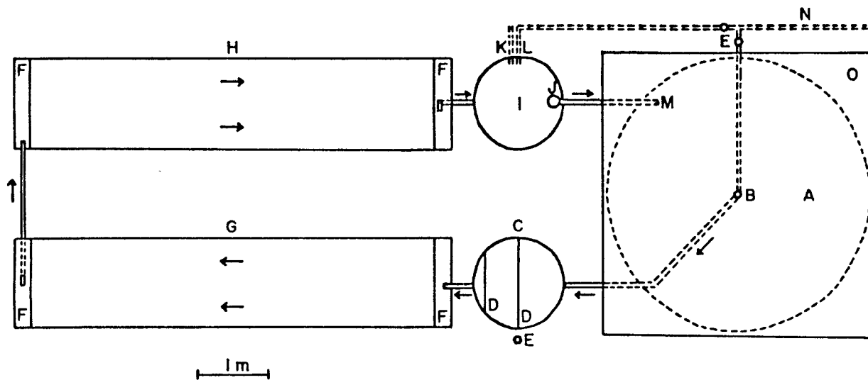
Figure 3. Plan view of a recirculating system for tilapia culture and vegetable hydroponics: A, rearing tank; B, outlet; C, clarifier; D, baffle; E, valve; F, sump; G, upper hydroponic biofilter; H, lower hydroponic biofilter; I, reservoir; J, pump; K, water inlet; L, overflow outlet; M, return inlet; N, drain line; O, canopy.
